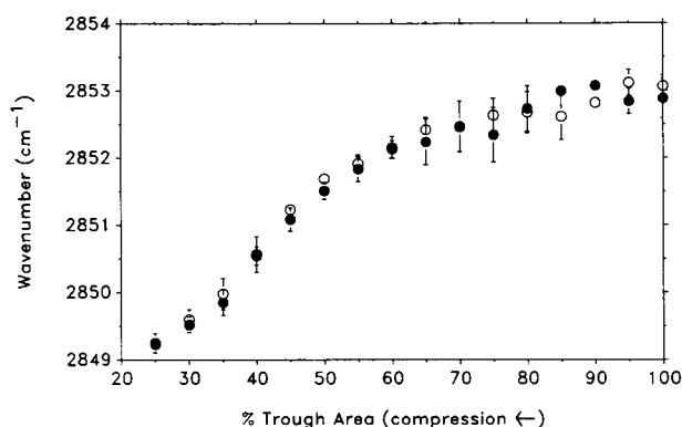
FIGURE 6 The frequency of the symmetric CH 2 stretching mode is plotted as a function of percentage of surface area for a surface film of bovine pulmonary surfactant at the A/W interface. Data was obtained for both perpendicular (●) and parallel (○) polarized spectra. The frequency-area isotherm was measured for a monolayer at 22°C by applying 5 \mu l of a 15-mg/ml solution of surfactant to the A/W interface of a 12.75 \times 23.10-cm Langmuir trough (20). Surface area for the heterogeneous surfactant monolayer was measured as a percentage of the initial trough surface area. The frequency was measured using a center-of-gravity algorithm.
