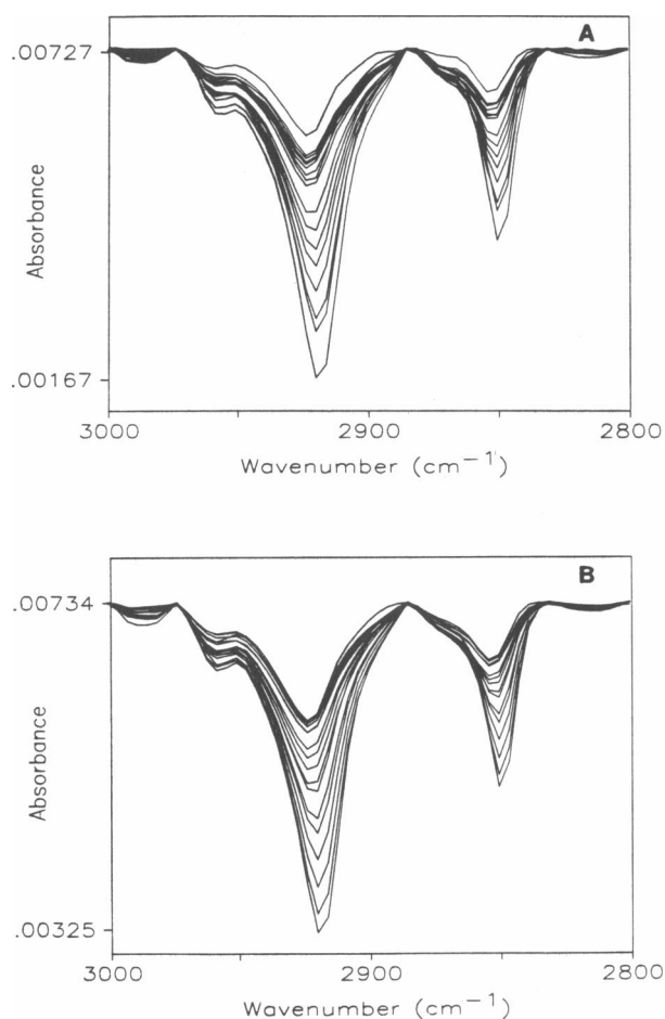
FIGURE 5 External reflection IR spectra of the raw bovine lung surfactant monolayer in the C-H stretching region. The CH 2 stretching bands are plotted for both (A) parallel and (B) perpendicular polarizations between 3,000 and 2,800 cm -1 . The spectra increase in intensity with increasing surface pressure. The surface pressure associated with each spectrum is given by the intermittently compressed data in Fig. 4, beginning with 0 dyn/cm and increasing to 37 dyn/cm. The band at ~2,920 cm -1 is the antisymmetric CH 2 stretch. The ~2,850-cm -1 band is the symmetric CH 2 stretch of the phospholipid hydrocarbon chains.
